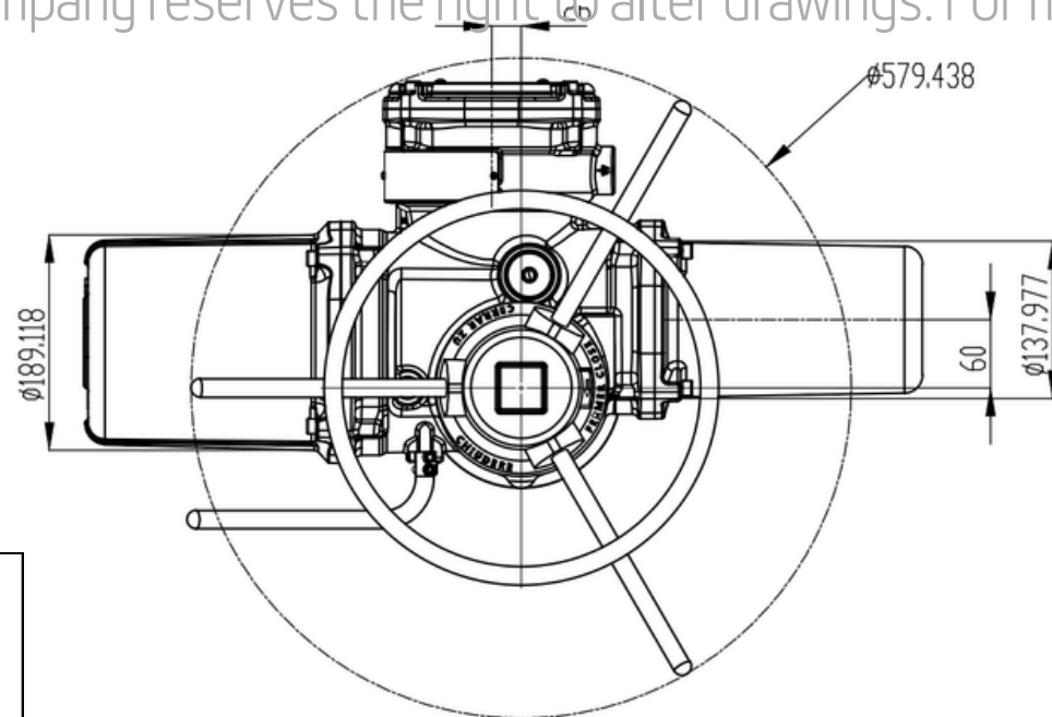
AVAMD Linear Electric Actuator Model: AVAMD 04 — F14
